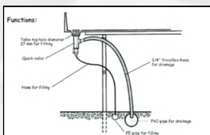
Quick valve
